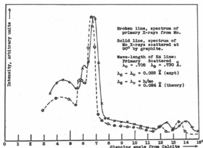
Fig. 10. Compton's spectra of 1923 for Molybdenum K_{\alpha} X rays scattered by graphite (carbon) through an angle of 90^{\circ} . Note that they are identical to those he published in October 1922 (Fig. 8), but that he now calculated the change in wavelength \lambda_0 - \lambda_s = h/mc between the secondary and primary light quantum on the basis of his new quantum theory of scattering. Source: Compton (1923), 495; Shankland (1975), p. 394.
